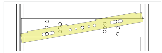
Installation option A - 10° inclined left
